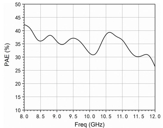
Power added efficiency vs. frequency (@ Pin=28dBm)
