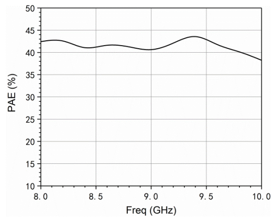
Power added efficiency vs. frequency (@ Pin=29dBm)
