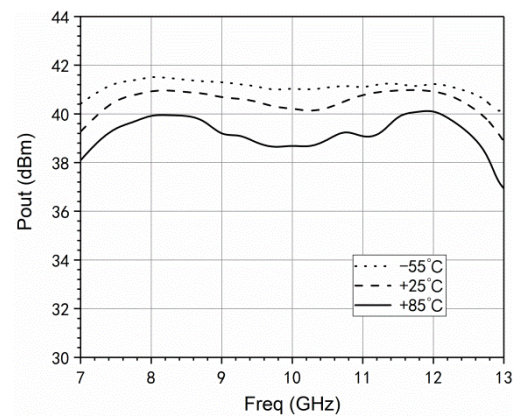
Three temperature output power vs. frequency (@Pin=21dBm)
