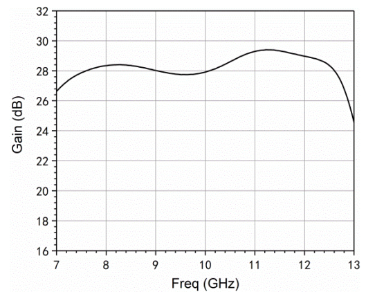
Small signal gain vs. frequency (@Pin=-10dBm)
