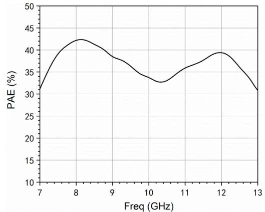
Power added efficiency vs. frequency(@Pin=21dBm)
