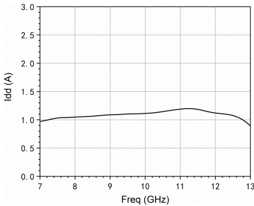
Dynamic current vs. frequency(@Pin=21dBm)
