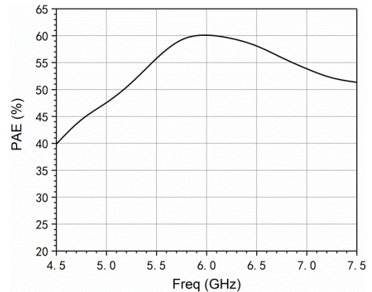
Power added efficiency vs. frequency(@Pin=22dBm)
