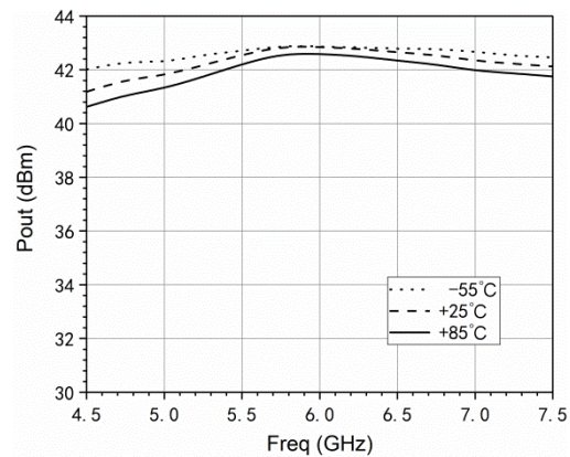
Three temperature output power vs. frequency (@Pin=22dBm)
