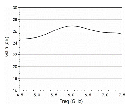
Small signal gain vs. frequency (@Pin=-25dBm)
