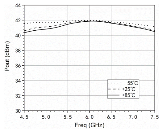
Three temperature output power vs. frequency (@Pin=20dBm)
