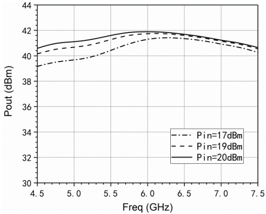
Output gain vs. frequency
