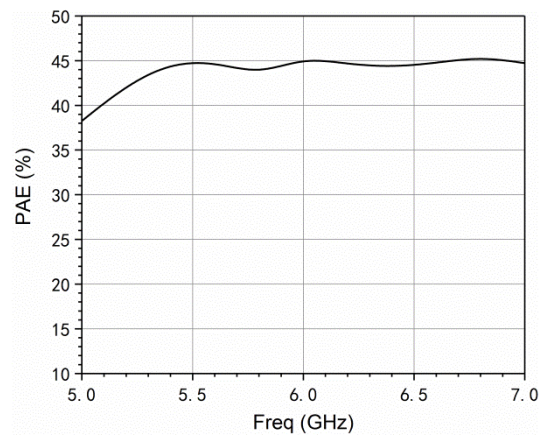
PAE vs. frequency (@ Pin=26dBm)
