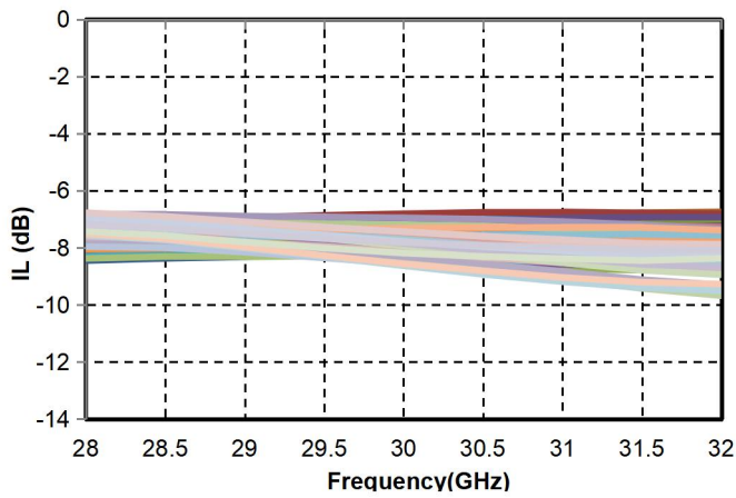
Appearance structure 2
