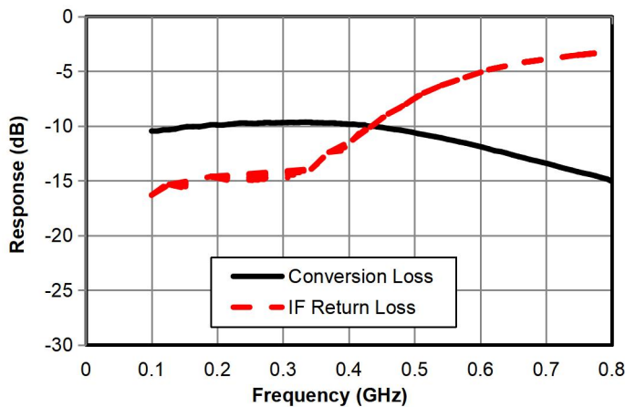
Intermediate frequency bandwidth @ LO=0.4G/+15dBm
