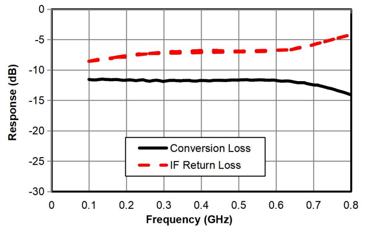
Intermediate frequency bandwidth @ LO=2G/+15dBm
