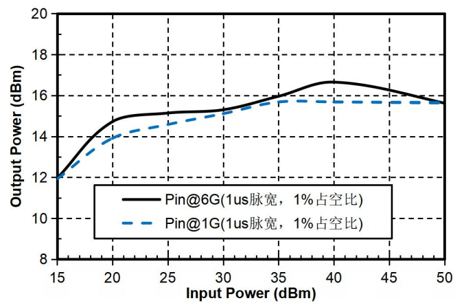
Limiting level @1G, 6G (1us pulse width, 1% duty cycle)
