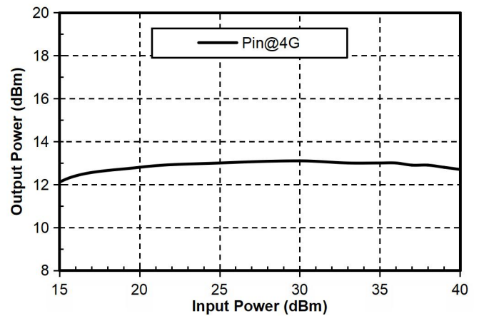
Clipping level@4GHz
