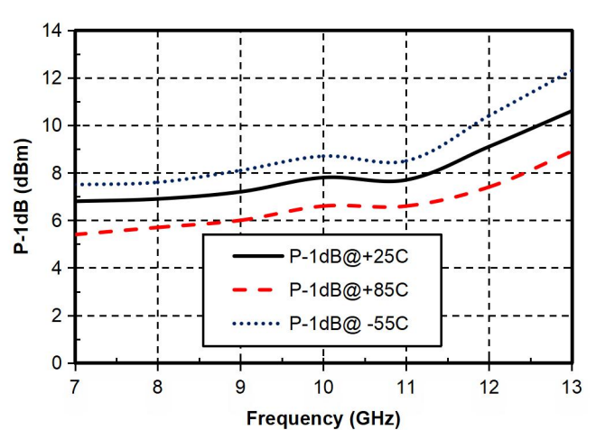
P-1dB vs. Temperature
