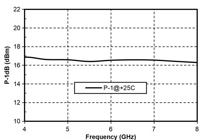
P-1dB vs. Temperature
