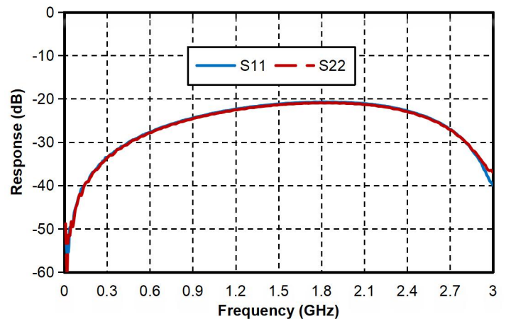
Input /Output Return Loss vs. Operating Frequency
