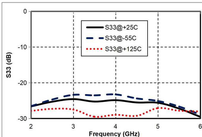
Coupled Output Return Loss vs. Operating Frequency
